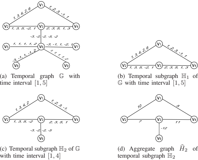
Fig. 1. Running example
